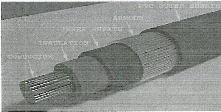
Fig . Typical power cable
